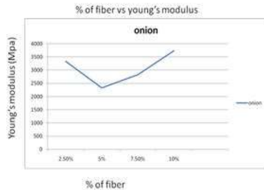
The variation of tensile stress and young's modulus of onion fiber reinforced Epoxy composites
