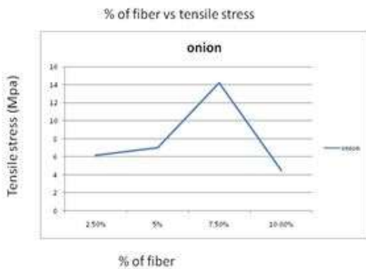
The variation of tensile stress and young's modulus of onion fiber reinforced Epoxy composites
