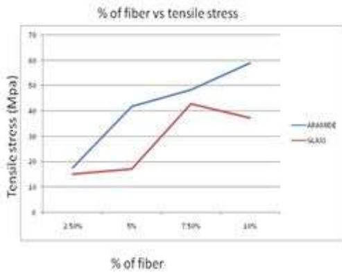
The variation of Stress with the ratio of Aramide and Glass fiber Reinforced Epoxy composites
