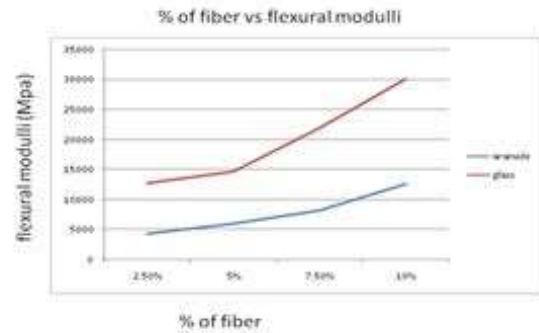
The variation of Flexural modulus with ratio of Aramide and Glass fibers reinforced Epoxy composites
